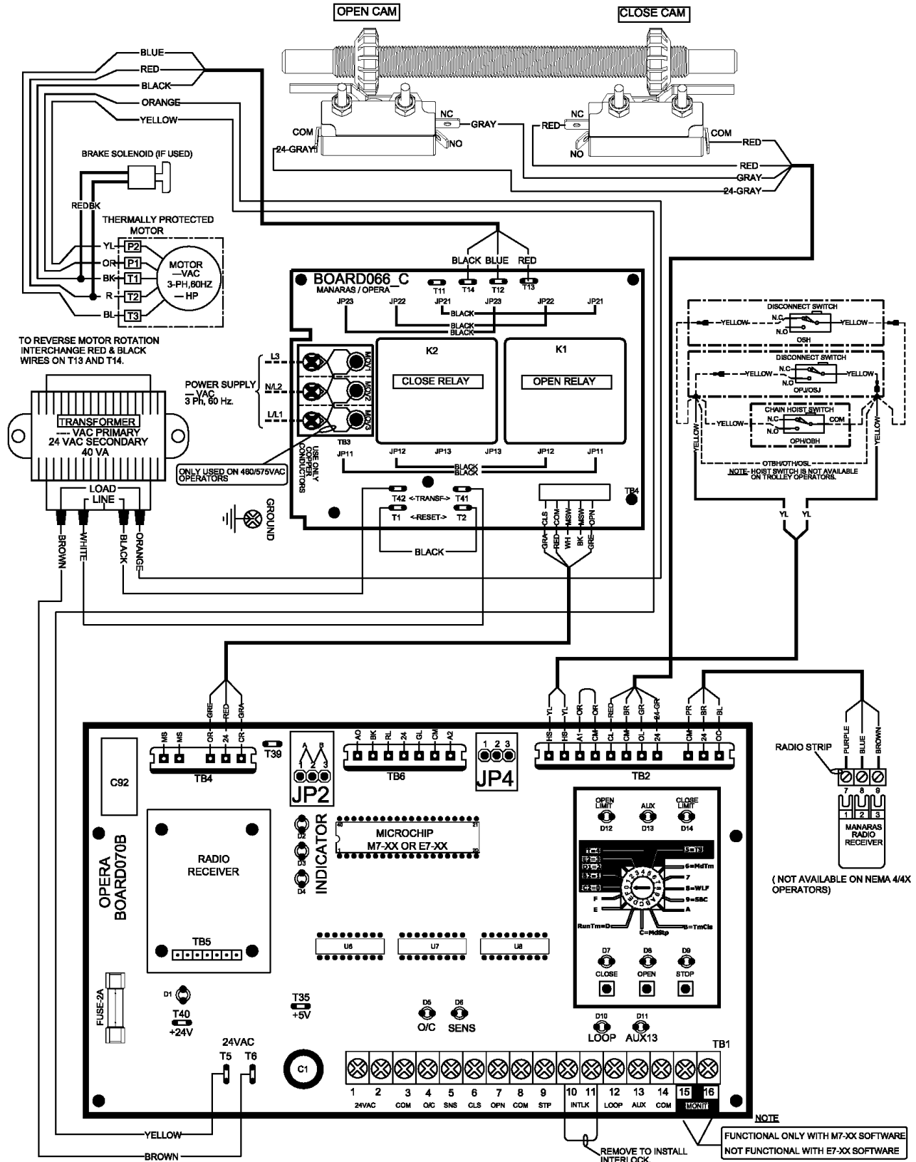
Figure 38 - EDWG1307006601
