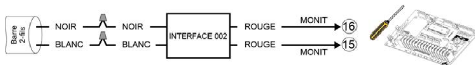
Figure 16 - Installation SENSEEDGE 007UM / 018UM / 044UM / 046M et INTERFACE 002
