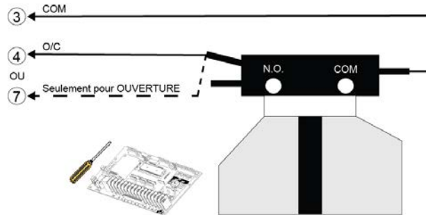
Figure 30 - PULLCORD 001 / 003 / 004 / 007
