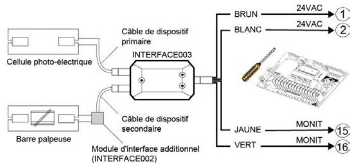
Figure 19 - Installation INTERFACE 003
