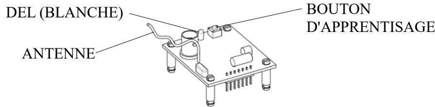
Figure 35: RADIOEM100 (ECB BOARD070)
