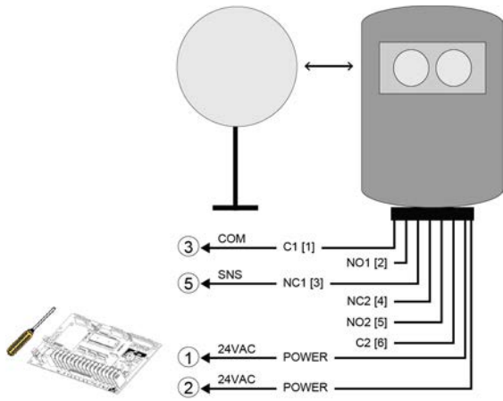
Figure 24 - PHOTO 018
