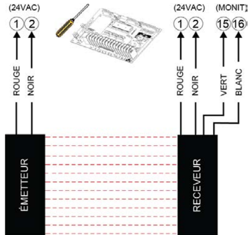
Figure 18 - Installation LIGHTCURTAIN 001 / 002
