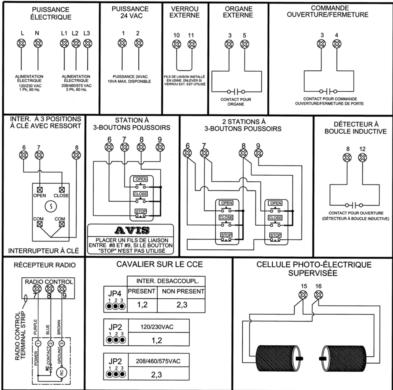
Figure 39 - Câblage externe
