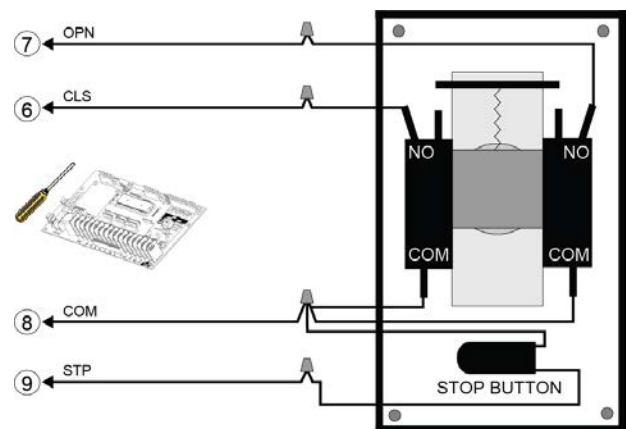
Figure 32 - KEYSWITCH 019
