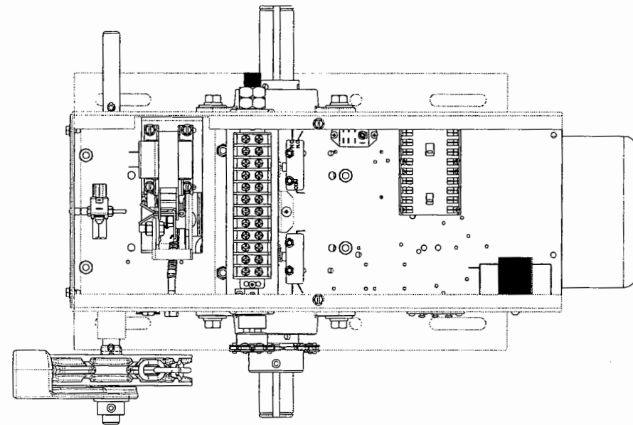
TOP AND ISO VIEWS SHOWN WITHOUT COVER001
