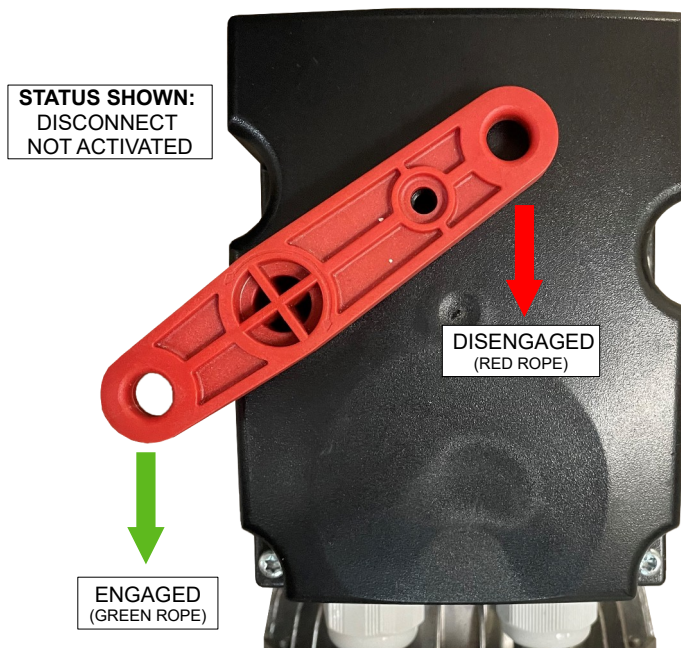
Figure 1- Disconnect Lever Mechanism
